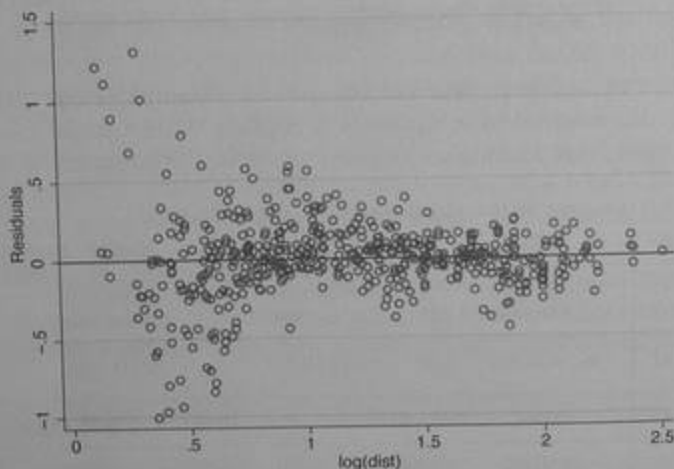
Figure 5.3: Residual-versus-predictor plot
